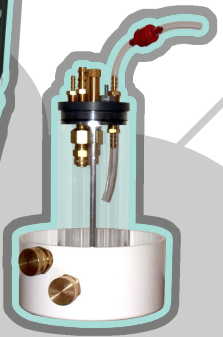
DRYSTIK with DCC Active humidity exchanger
